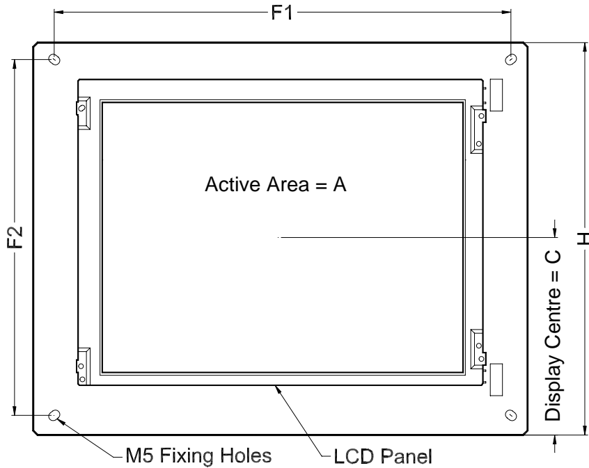
REAR VIEW
