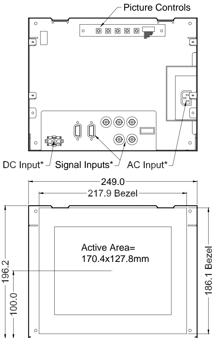
FRONT VIEW
