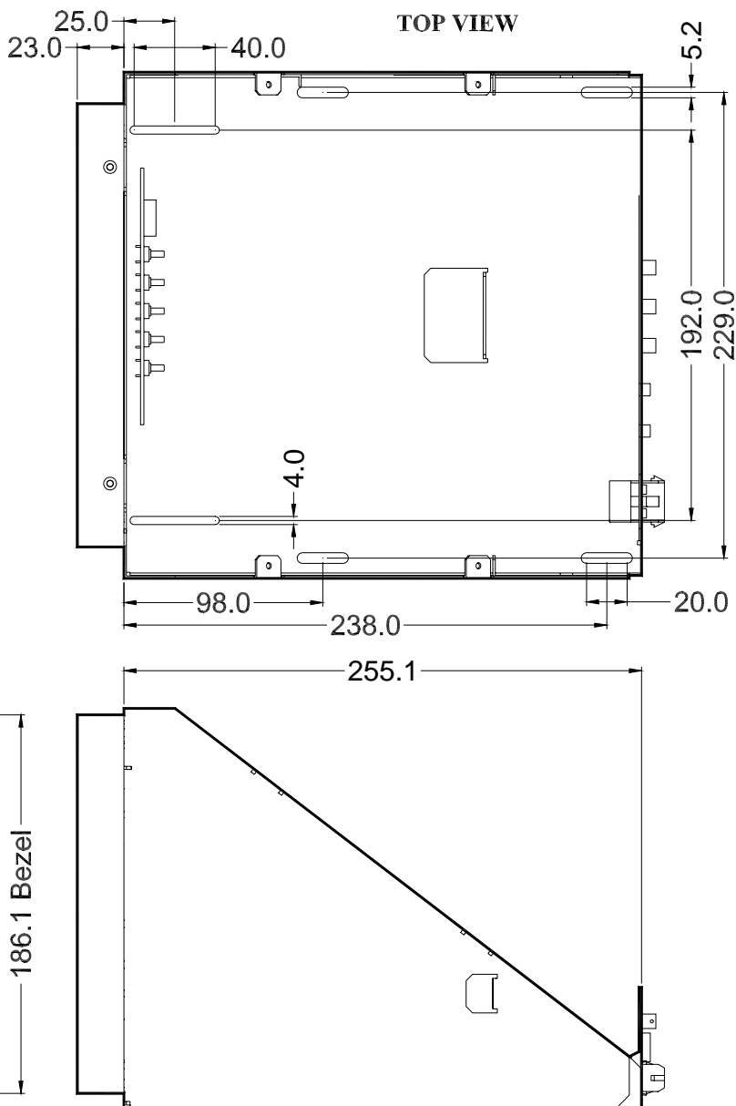
SIDE VIEW
